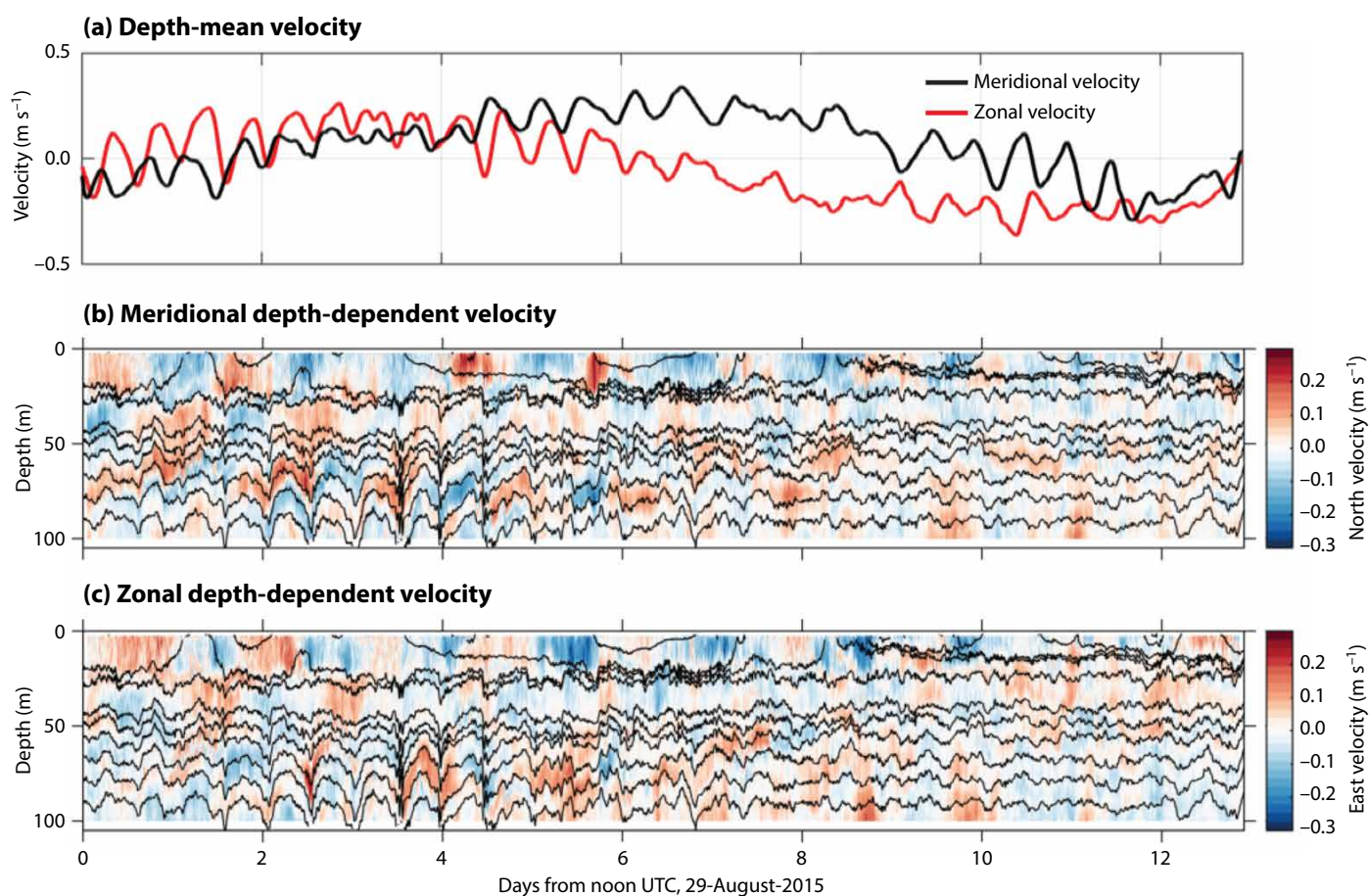
FIGURE 3. Along-track time series of (a) depth-mean meridional and zonal velocities, (b) depth-dependent meridional velocities, and (c) depth-dependent zonal velocities from a single point current meter affixed to the Wirewalker profiler. Depth-mean velocities were dominated by the mesoscale and semidiurnal fluctuations associated with a propagating low-mode internal tide. Depth-dependent velocities, and thus shear, showed the imprint of energetic near-inertial oscillations with upward phase propagation in the thermocline. Near-inertial shear was enhanced at the base of the mixed layer but not at the interface between the barrier layer and the stratified interior. This decoupling between the upper ocean and the thermocline may be due to the characteristic two (or more) layer stratification of the Bay of Bengal.
